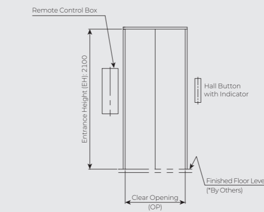
E050 TYPE WITH CP IN HOISTWAY
