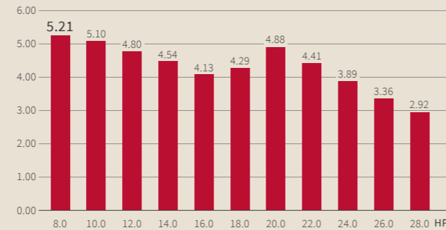
Heating COP
